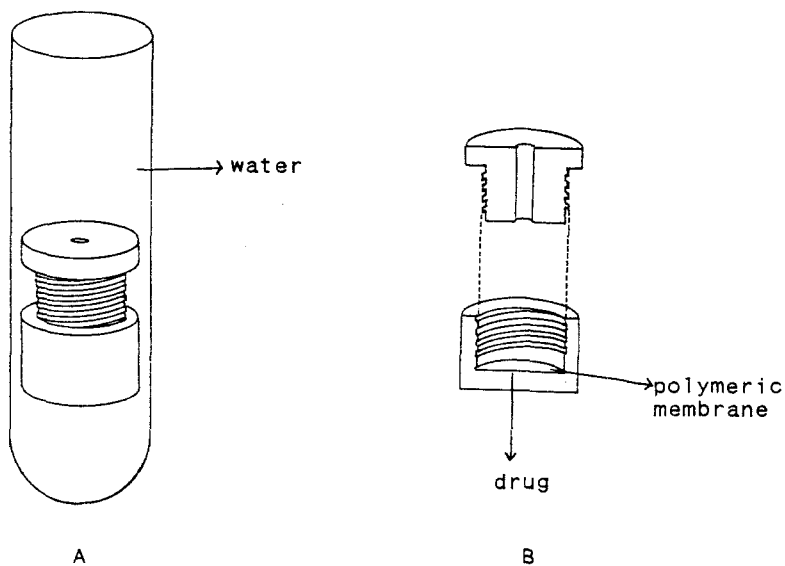
A - Device placed inside the glass tube. B - Longitudinal cut of the device.
